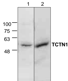
Cat. #: 3088-100 TCTN1 Antibody. Western blot analysis of TCTN1 using Jurkat cell lysate (Lane 1) and rat kidney tissue lysate (Lane 2).
